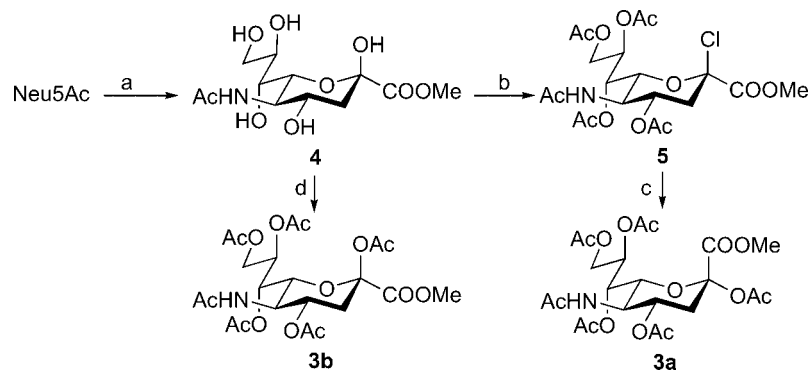
Scheme 2. Preparation of Neu5Ac peracetates 3a and 3b . a) MeOH, Dowex H + , room temperature, 24 h; b) HCl, AcOH/AcCl (1:1), room temperature; c) CsOAc (1.5 equiv.), MeCN, room temperature; 74% from Neu5Ac; d) Ac 2 O, pyridine, room temperature, overnight ( 3a/3b ≈ 1:4 \alpha/\beta mixture); flash column chromatography on silica gel; 74% of 3b from Neu5Ac.
