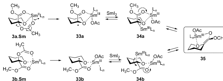
Scheme 5. Postulated mechanism for the formation of the samarium enolate from 3a and 3b .
