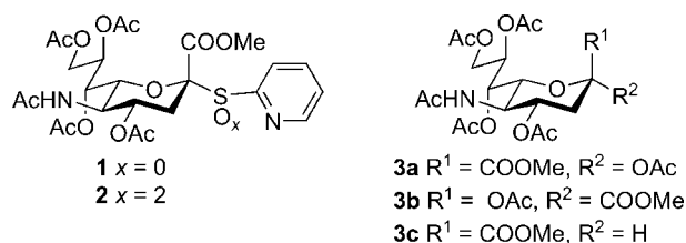
Figure 1. Structure of Neu5Ac derivatives.
