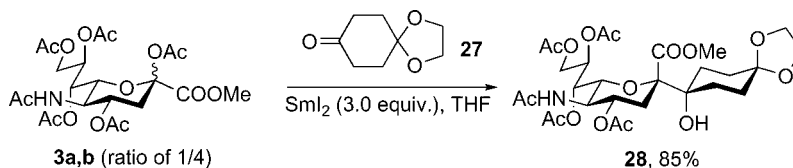
Scheme 3. Coupling reaction with 4-dioxolanocyclohexanone 27 .
