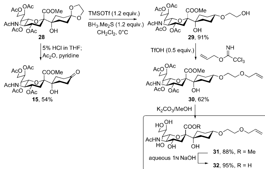
Scheme 4. Selective synthesis of the C-sialoside building block 32 .
